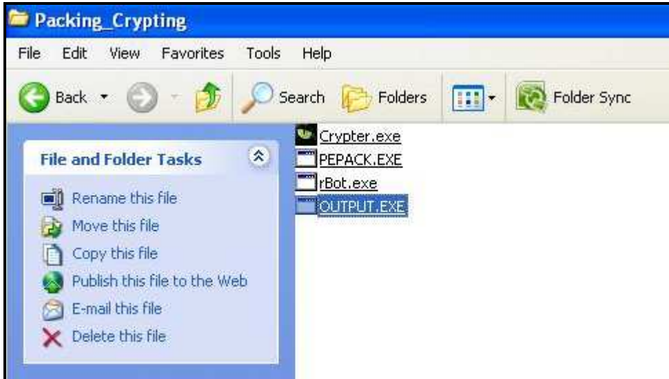
Figure 6.2: OUTPUT.EXE
